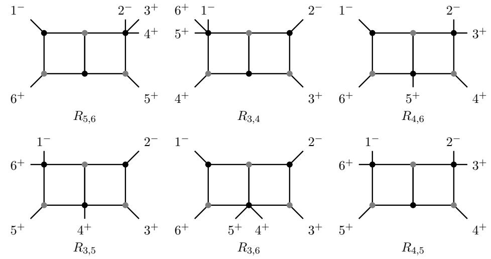
Figure 1. On-shell diagrams giving rise to leading singularities R_{i,j} , for the --++++ helicity configuration.
